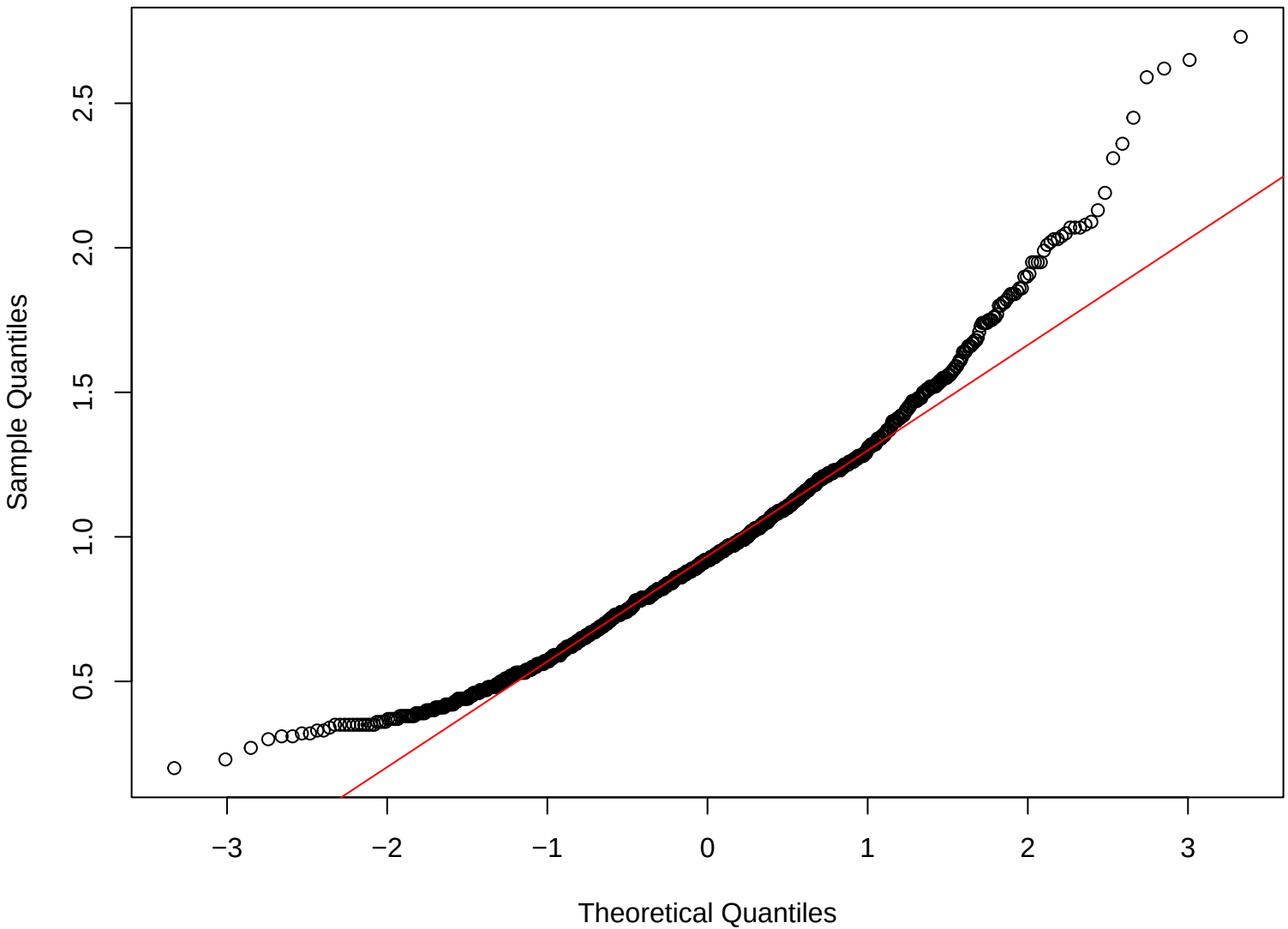
Q-Q Plot: lipids1
