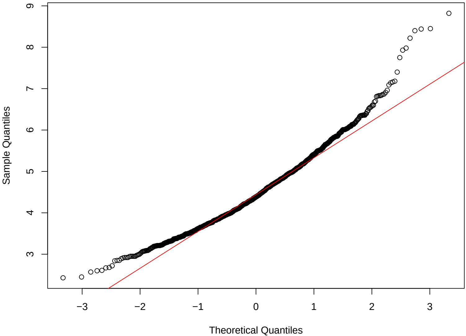
Q-Q Plot: lipids2
